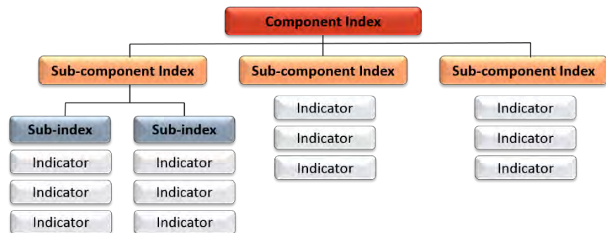
Figure 6. Index hierarchy
